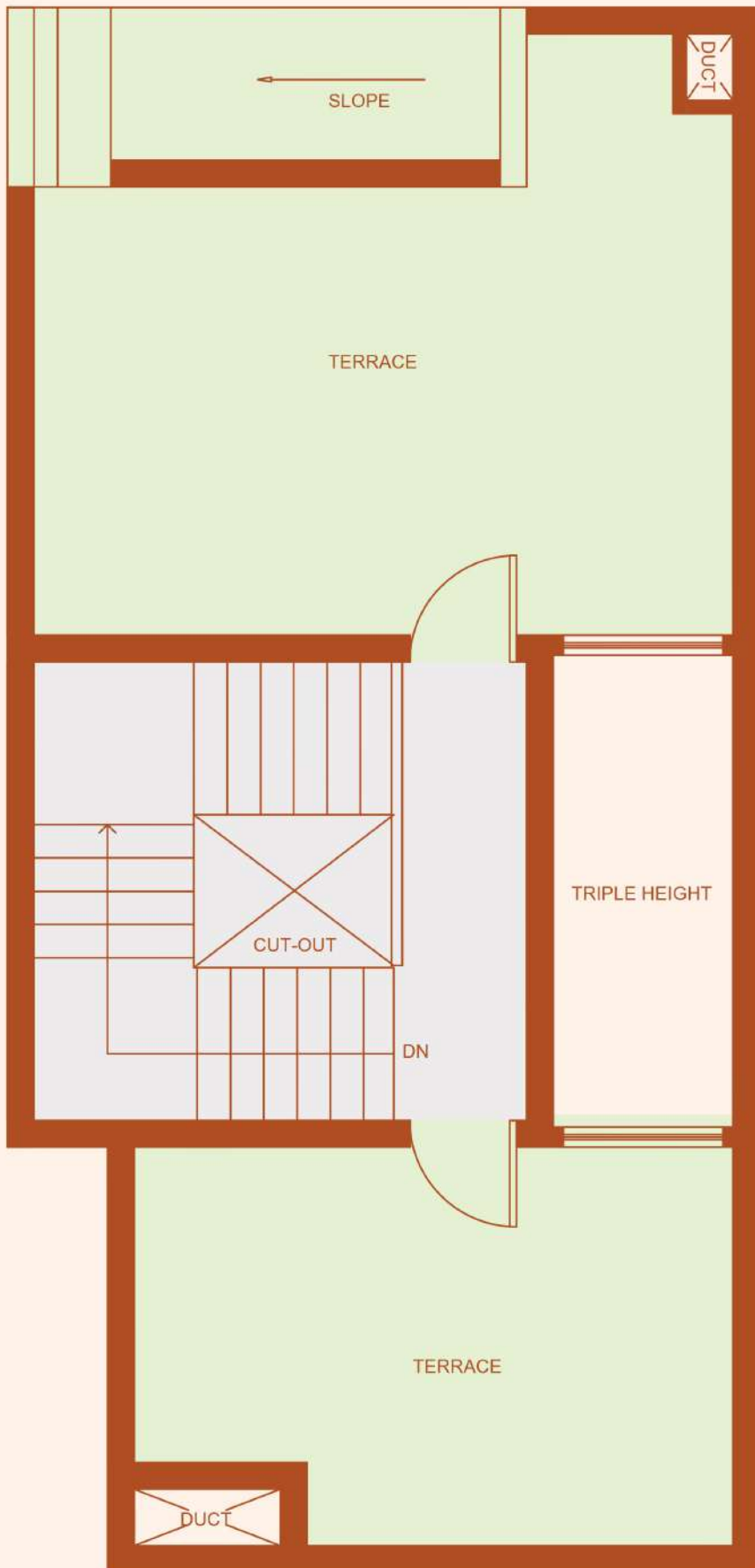
ROOFTOP PLAN
